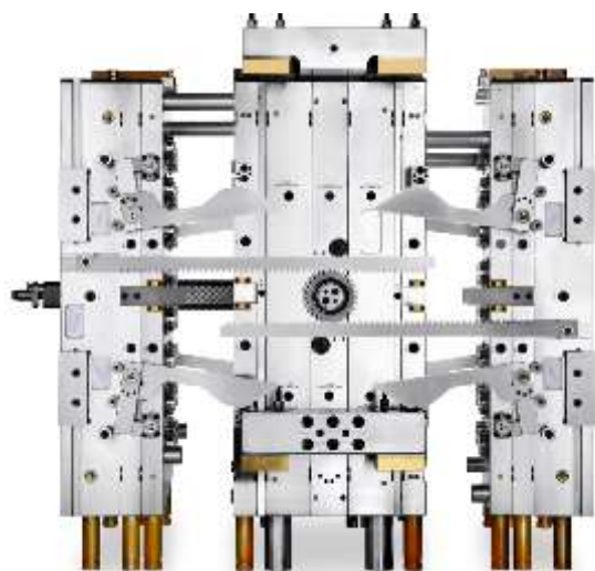
Stack Mold
